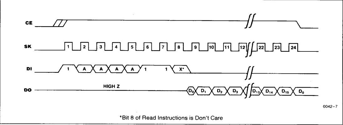
Figure 1: RAM Read
