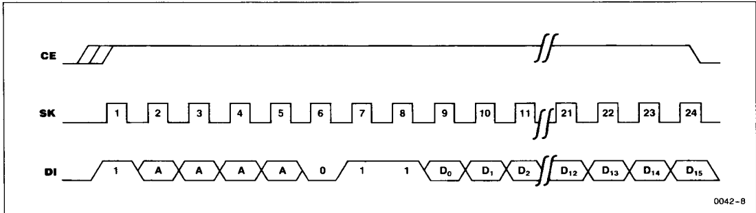
Figure 3: Non-Data Operations
