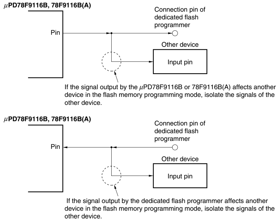
Figure 6-6. Abnormal Operation of Other Device
