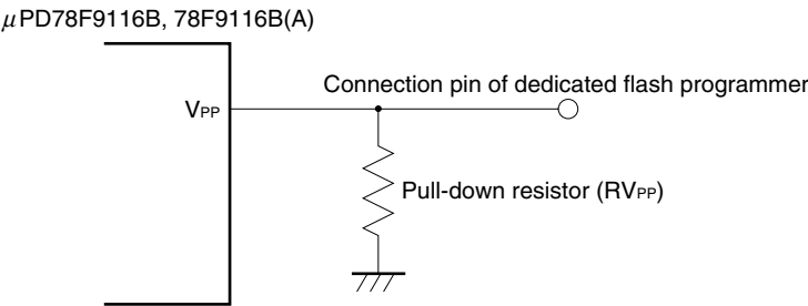
Figure 6-4. V PP Pin Connection Example
