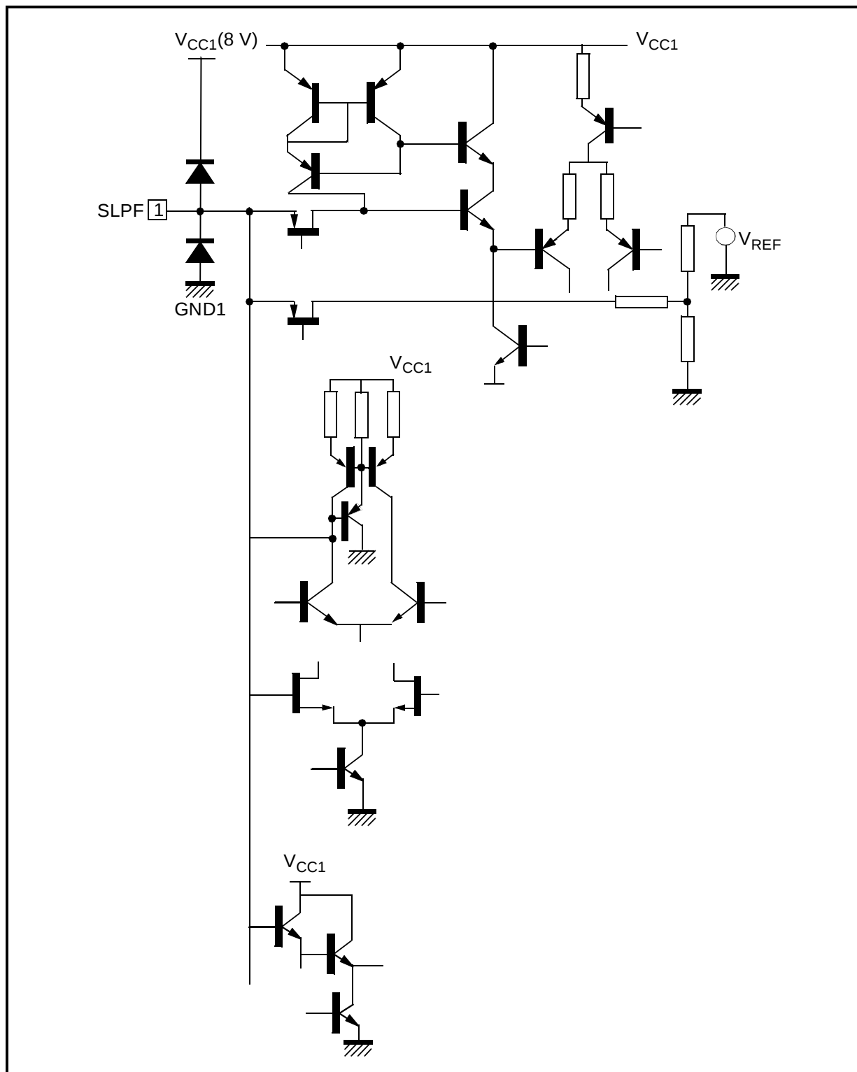
Figure 20. STV2238D (TQFP64)
