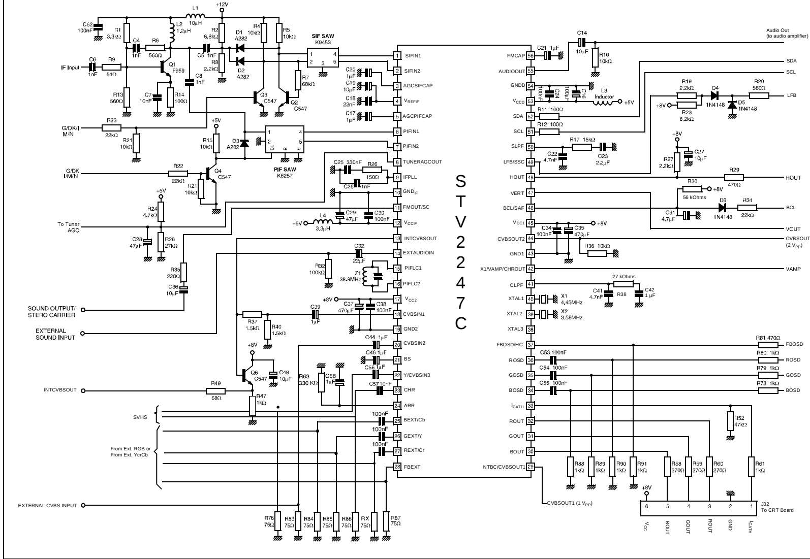
Figure 39. STV2247C
