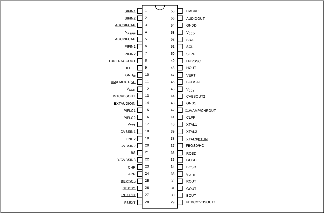
Figure 1. STV224XC/8XC Pinout (SDIP56)
