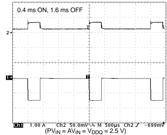
Upper Trace: VTT Output Waveform, 50 mV/Division, AC Coupled Lower Trace: Loading Current, IVTT, 1 A/Division ( PV_{IN} = AV_{IN} = V_{DDQ} = 2.5\text{ V} )
