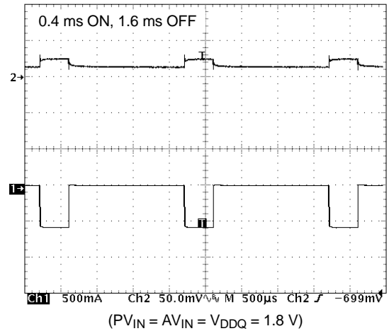
Upper Trace: VTT Output Waveform, 50 mV/Division, AC Coupled Lower Trace: Loading Current, IVTT, 500 mA/Division ( PV_{IN} = AV_{IN} = V_{DDQ} = 1.8\text{ V} )
