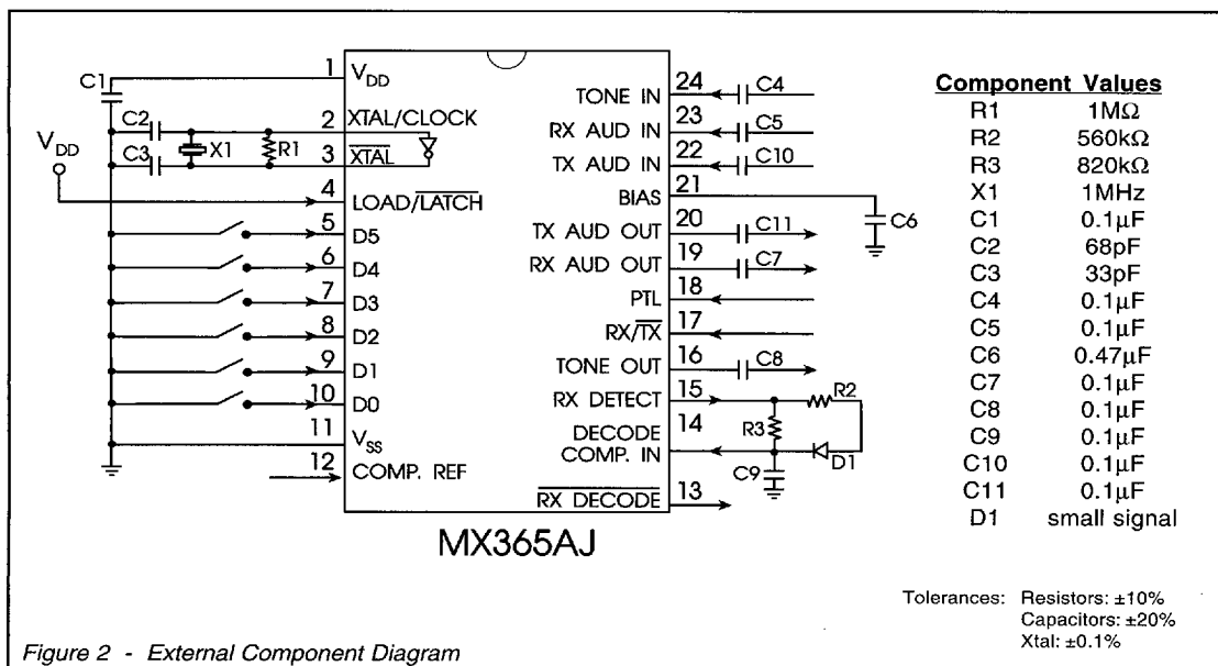
Figure 2 - External Component Diagram
