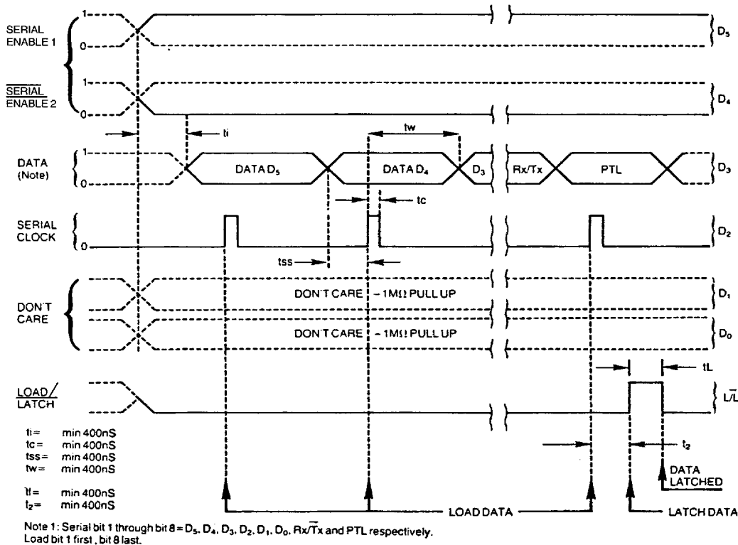
Figure 5 - Serial Mode (not to scale)
