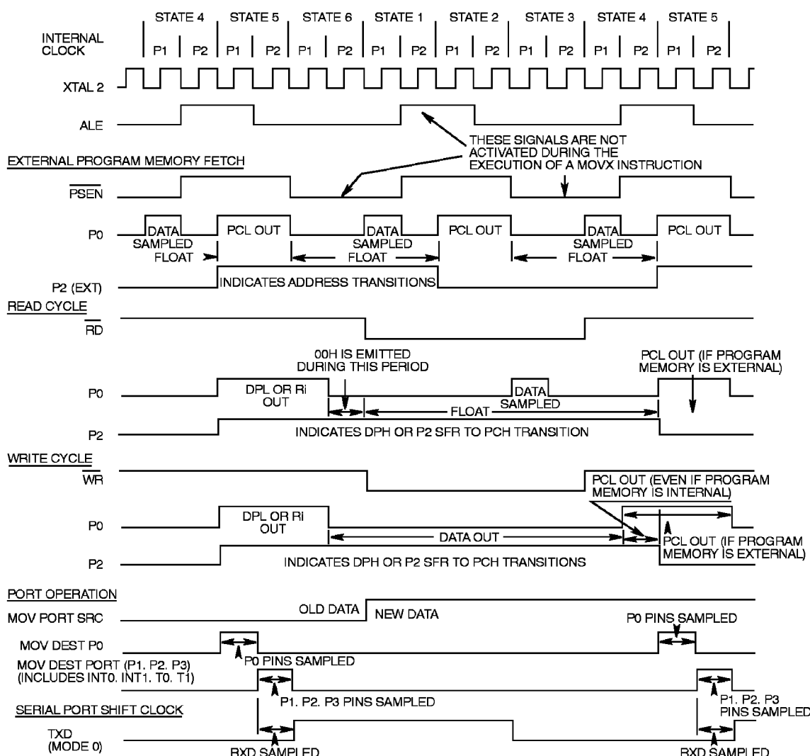
Figure 20. Clock Waveforms
