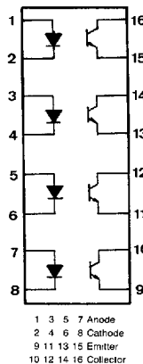
Pin No. and internal connection diagram
