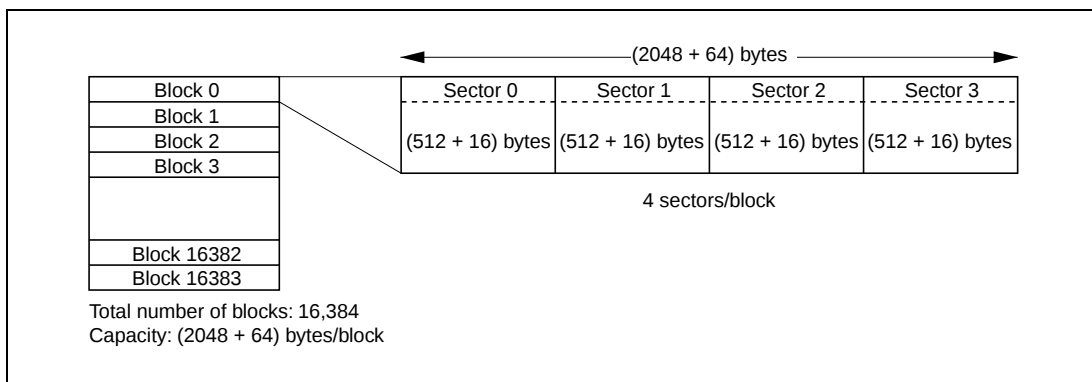
Figure 6.1 Flash Configuration
