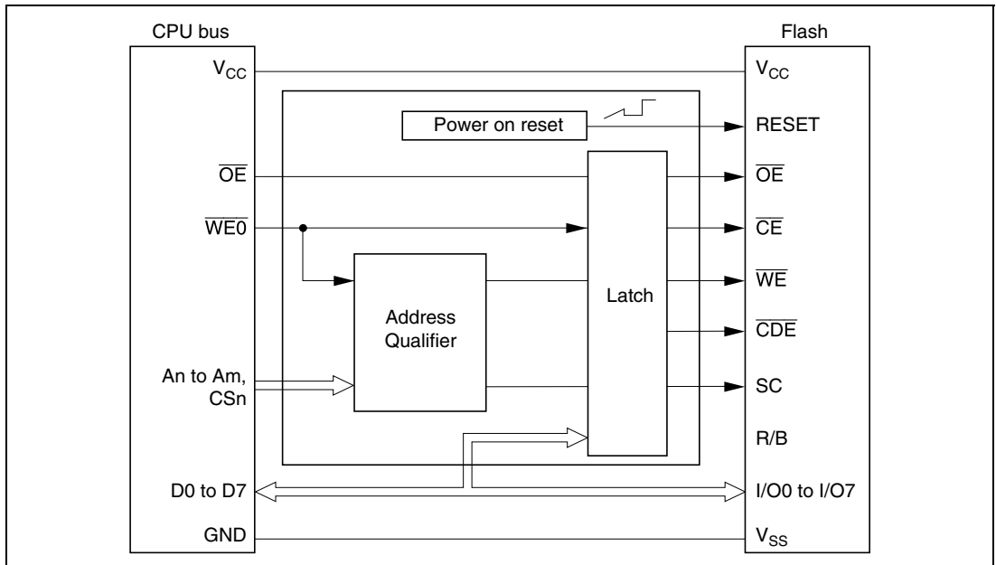
Figure 4.2 Flash Memory Interface Block Configuration
