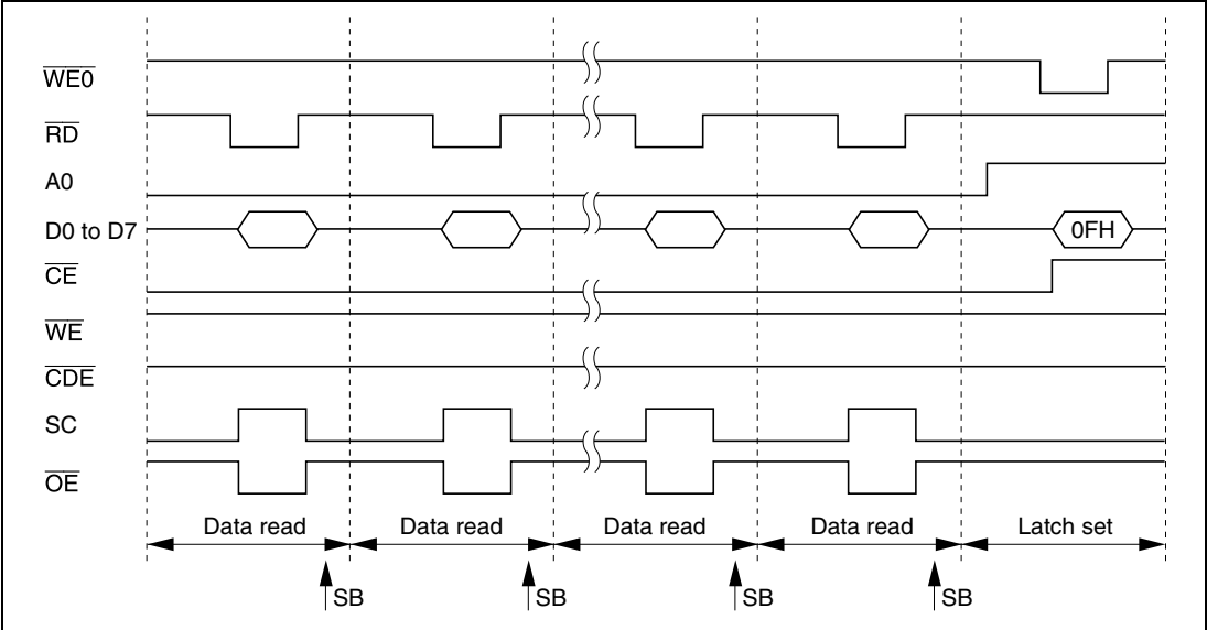
Figure 4.5 Example of Read Timing Waveforms
