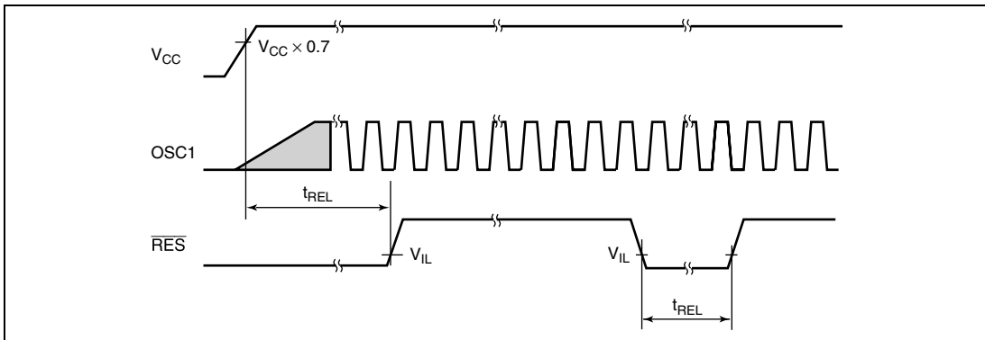
Figure 20.2 \overline{\text{RES}} Low Width Timing
