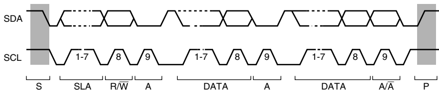
Figure 15.4 I 2 C Bus Timing
