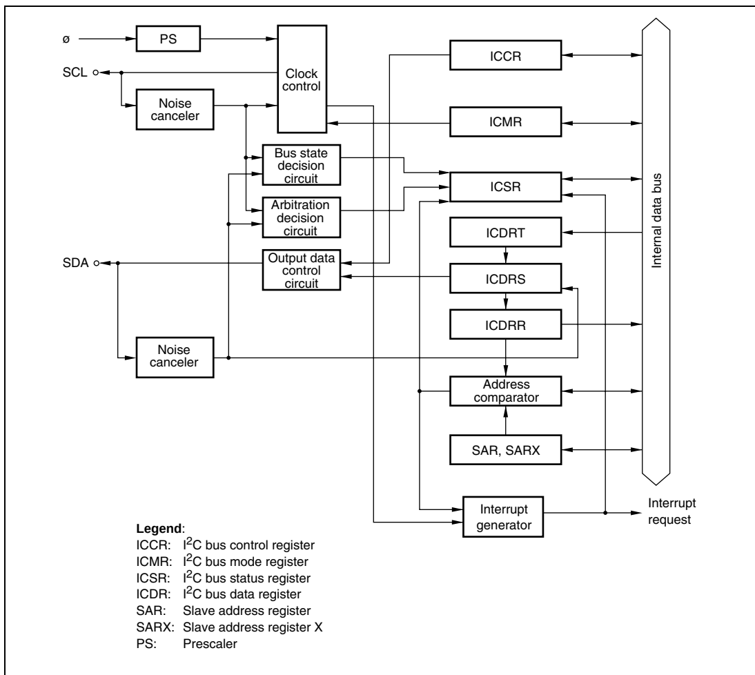
Figure 15.1 Block Diagram of I²C Bus Interface
