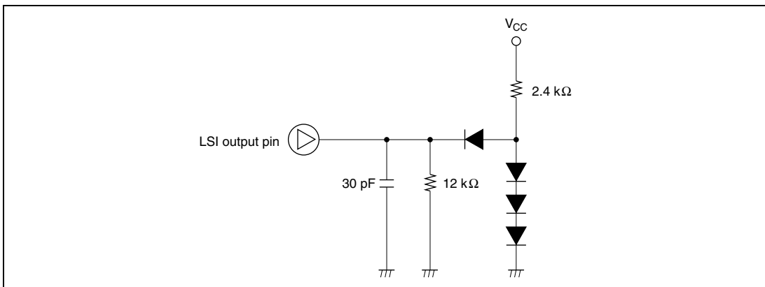
Figure 20.8 Output Load Circuit
