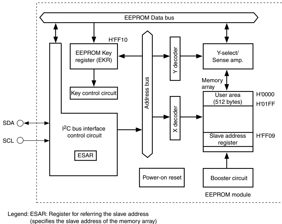
Figure 17.1 Block Diagram of EEPROM
