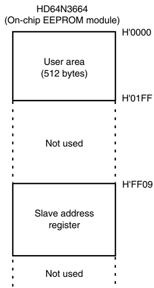
Figure 2.1 Memory Map (3)
