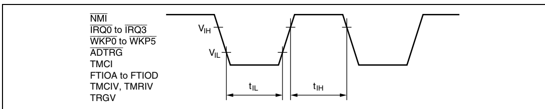
Figure 20.3 Input Timing
