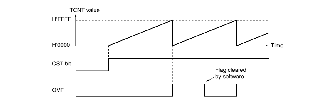
Figure 12.2 Free-Running Counter Operation
