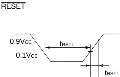
Figure 81 Reset Timing
