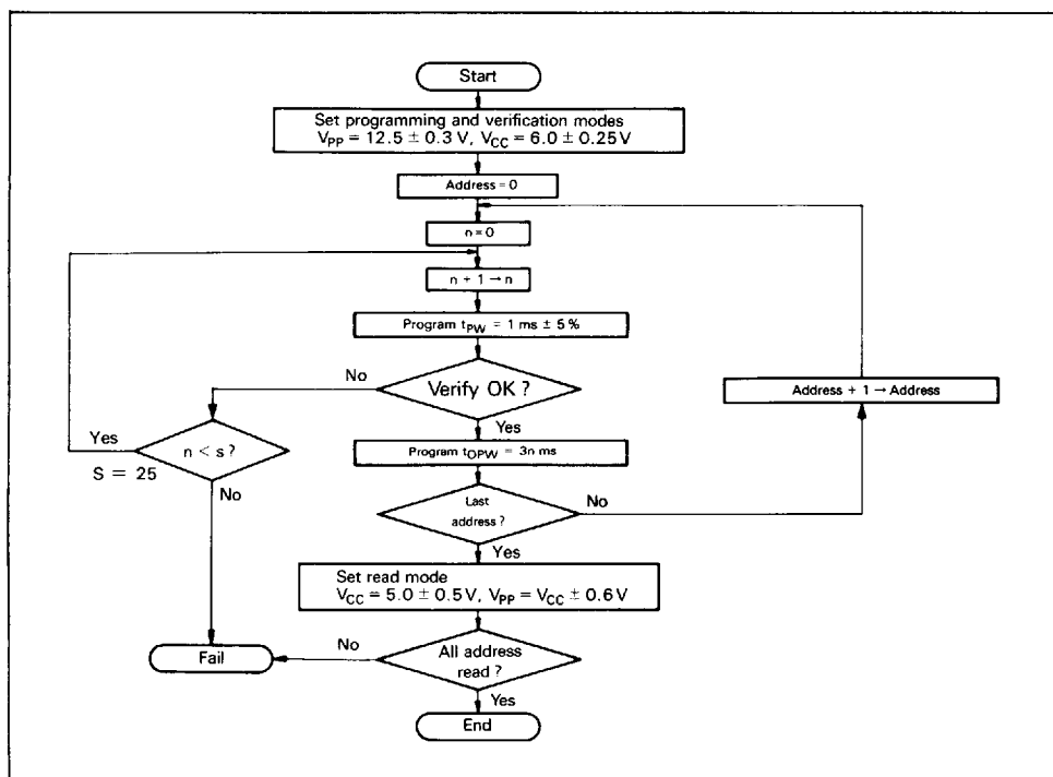
Figure 24 PROM Programming
