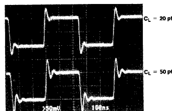
Pulse Response with V_+ = 15V, V_- = -15V
