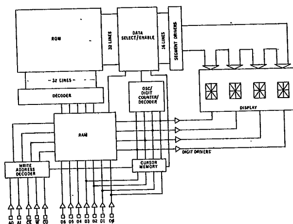
INTERNAL SCHEMATIC
