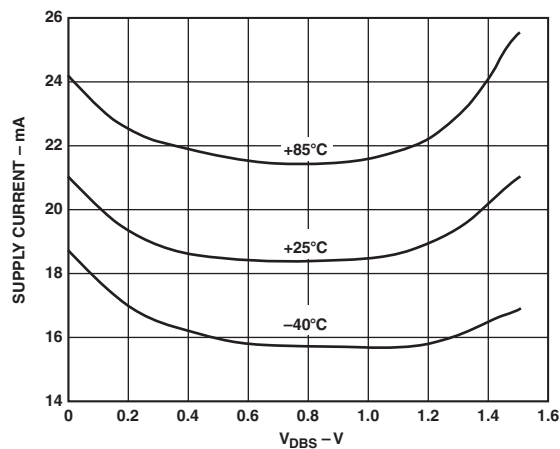
TPC 40. Supply Current vs. V_{DBS} at Three Temperatures
