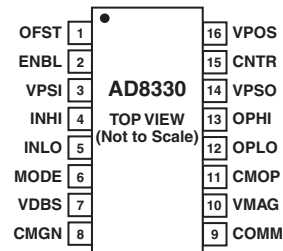
16-Lead QSOP
