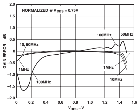
TPC 4. Gain Error vs. V_{DBS} at Various Frequencies
