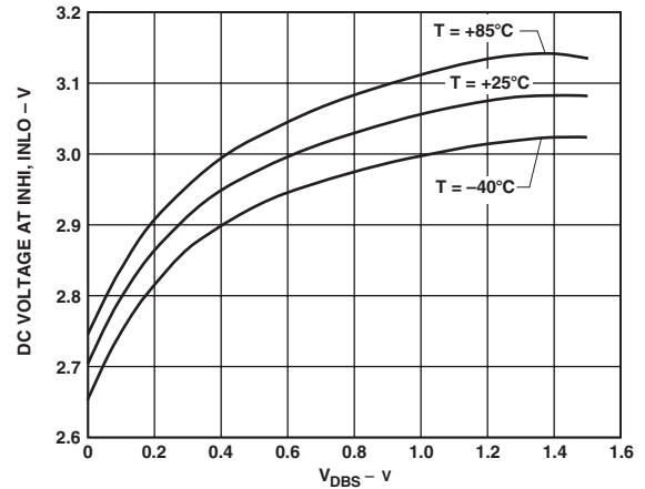
Figure 12. Common-Mode Voltage at Input Pins vs. V_{\text{DBS}} , for V_S = 5 V, T = -35^\circ\text{C} , +25^\circ\text{C} , and +85^\circ\text{C}
