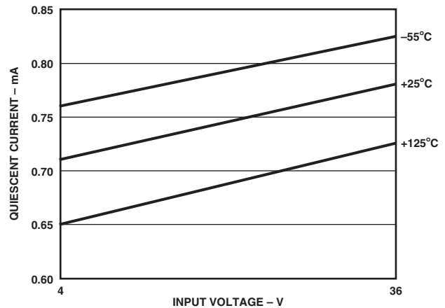
Figure 10. Typical Supply Current over Temperature
