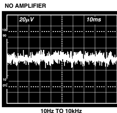
Figure 6. Reduced Noise Performance with C1 = 100 \mu F , C2 = 100 nF
