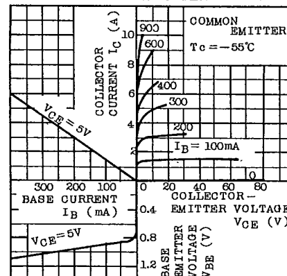
I_C - V_{CE} (LOW VOLTAGE REGION)
