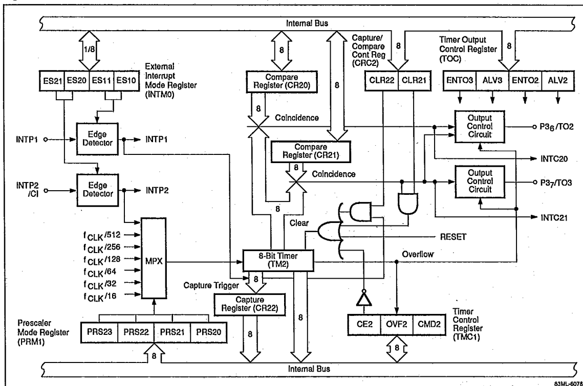
Figure 9. 8-Bit Timer/Counter 2
