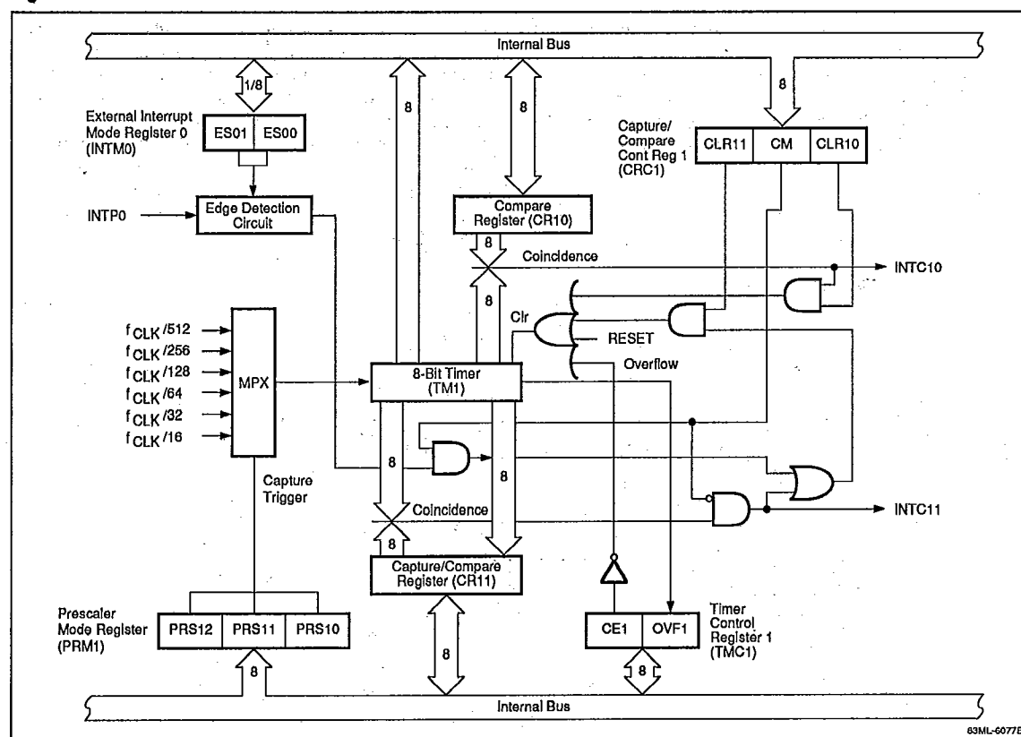
Figure 8. 8-Bit Timer/Counter 1
