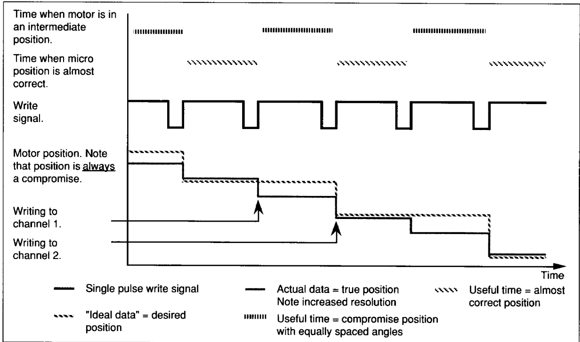
Figure 12. Single pulse programming, in- and output signals.
