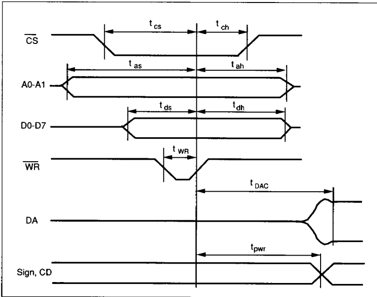
Figure 2. Timing.
