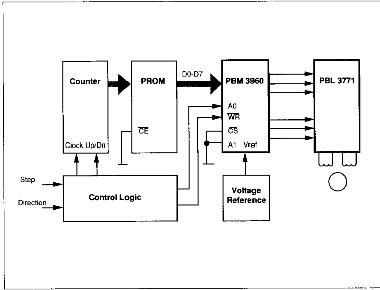
Figure 13. Typical block diagram of an application without a microprocessor. Available as testboard, TB 3071.
