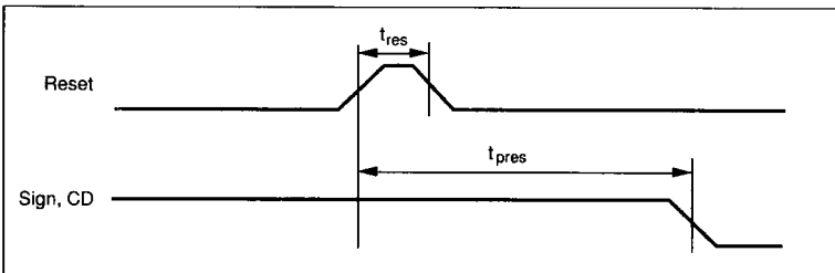
Figure 3. Timing of Reset.
