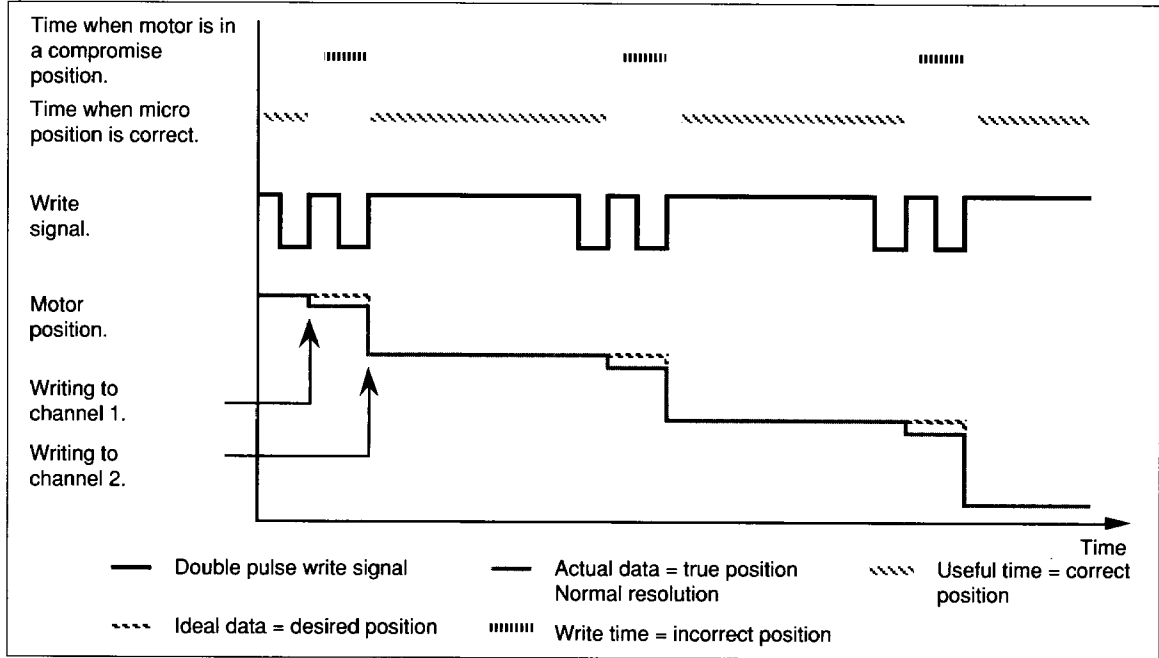
Figure 11. Double pulse programming, in- and output signals.
