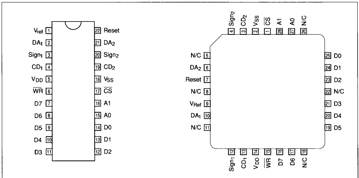
Figure 4. Pin configuration.
