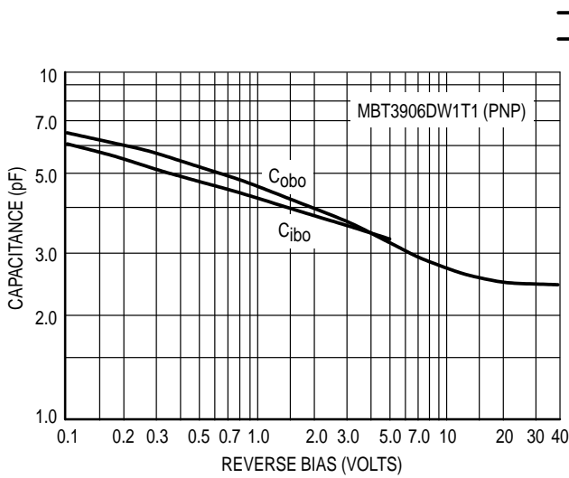
Figure 21. Capacitance
