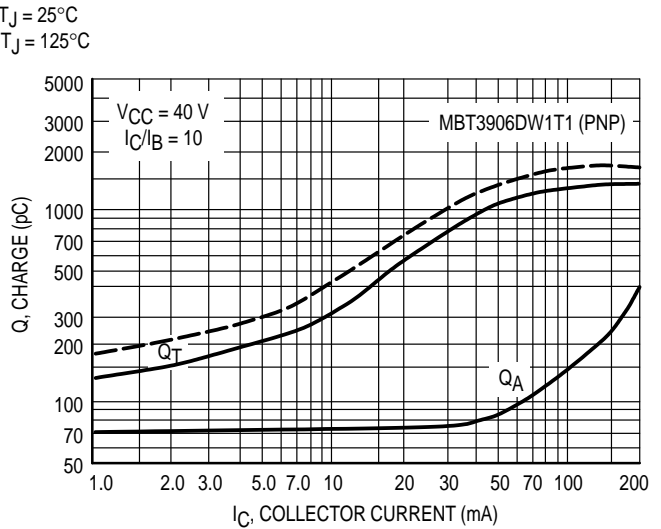
Figure 22. Charge Data
