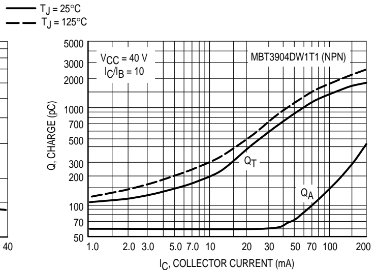
Figure 4. Charge Data
