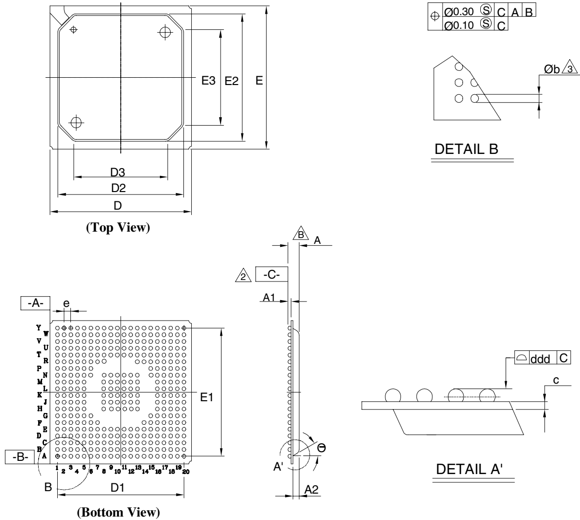
Figure 38. 352 Pin PBGA Pin Diagram
