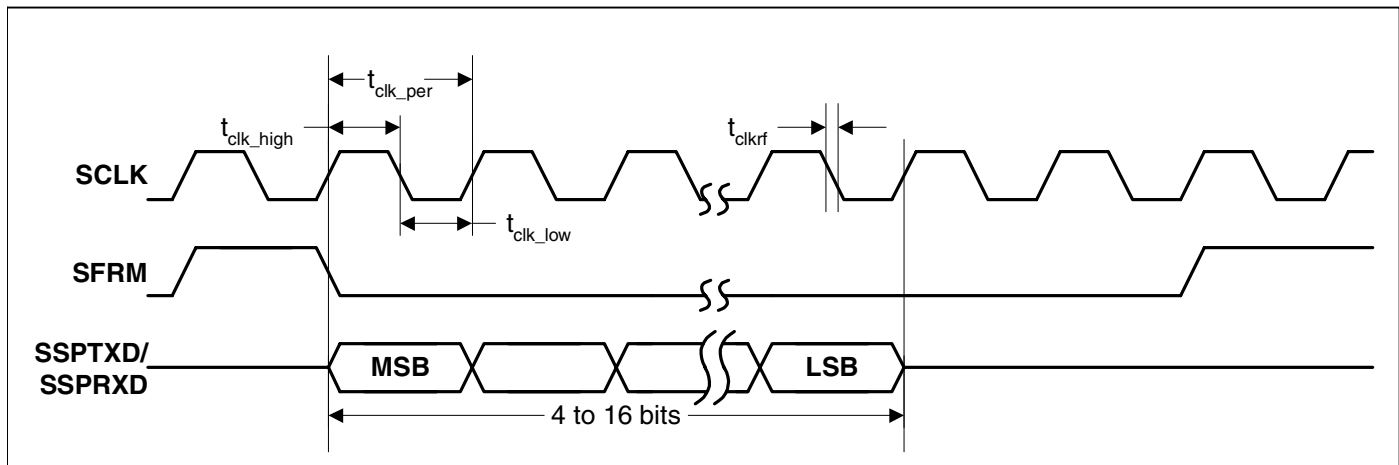
Figure 30. SPI Single Transfer Timing Measurement
