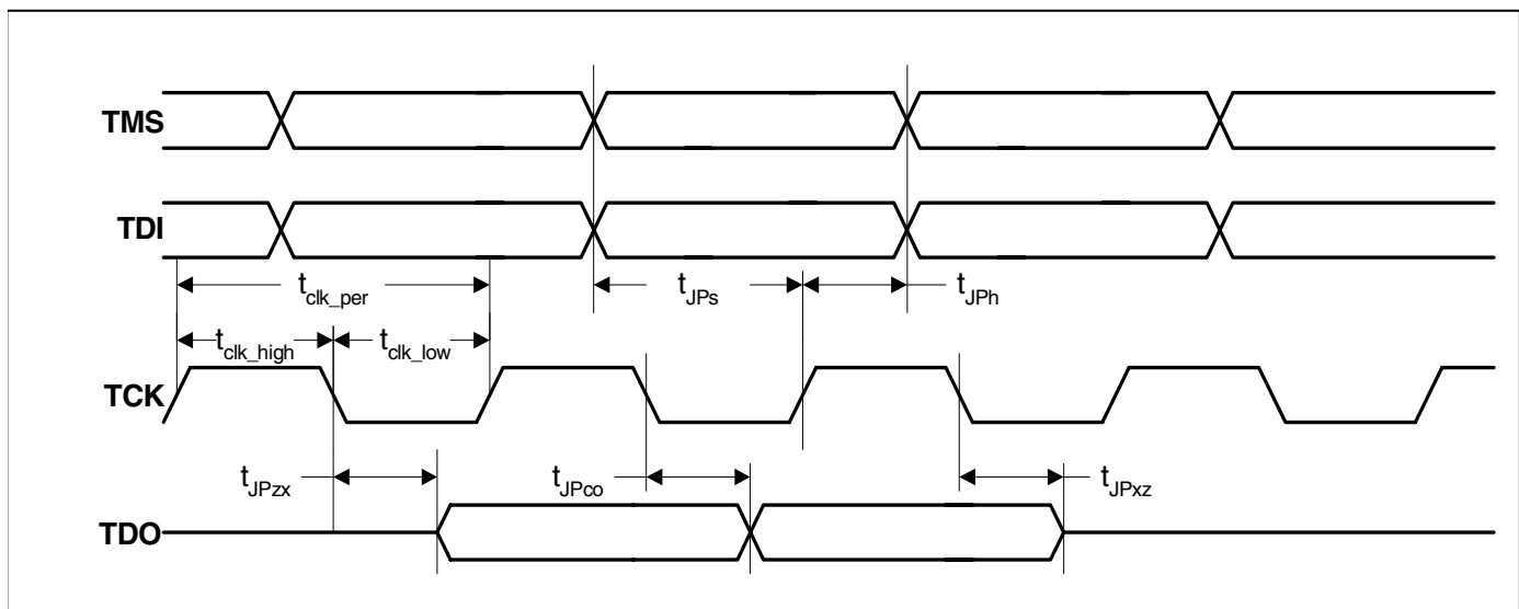
Figure 37. JTAG Timing Measurement
