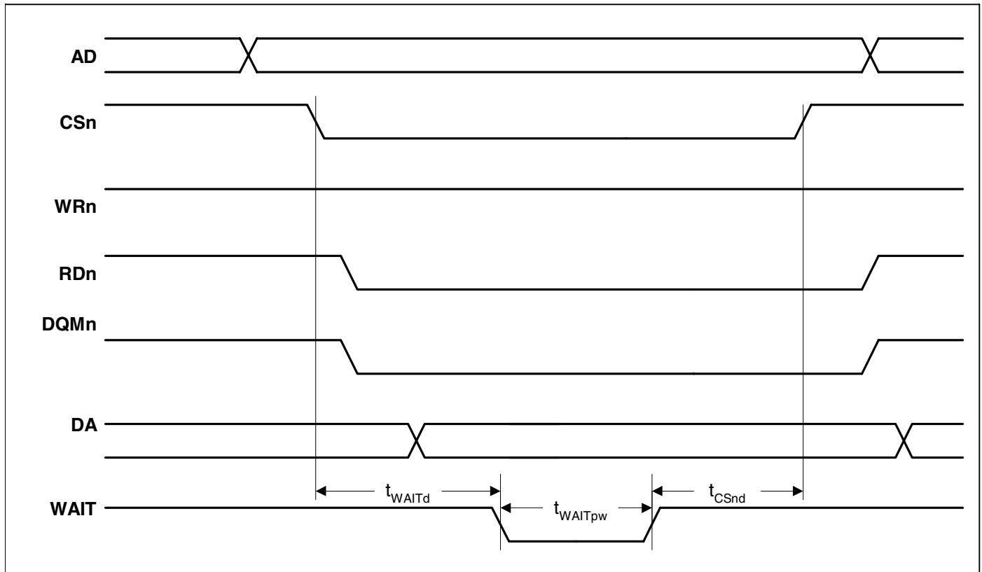
Figure 13. Static Memory Single Read Wait Cycle Timing Measurement
