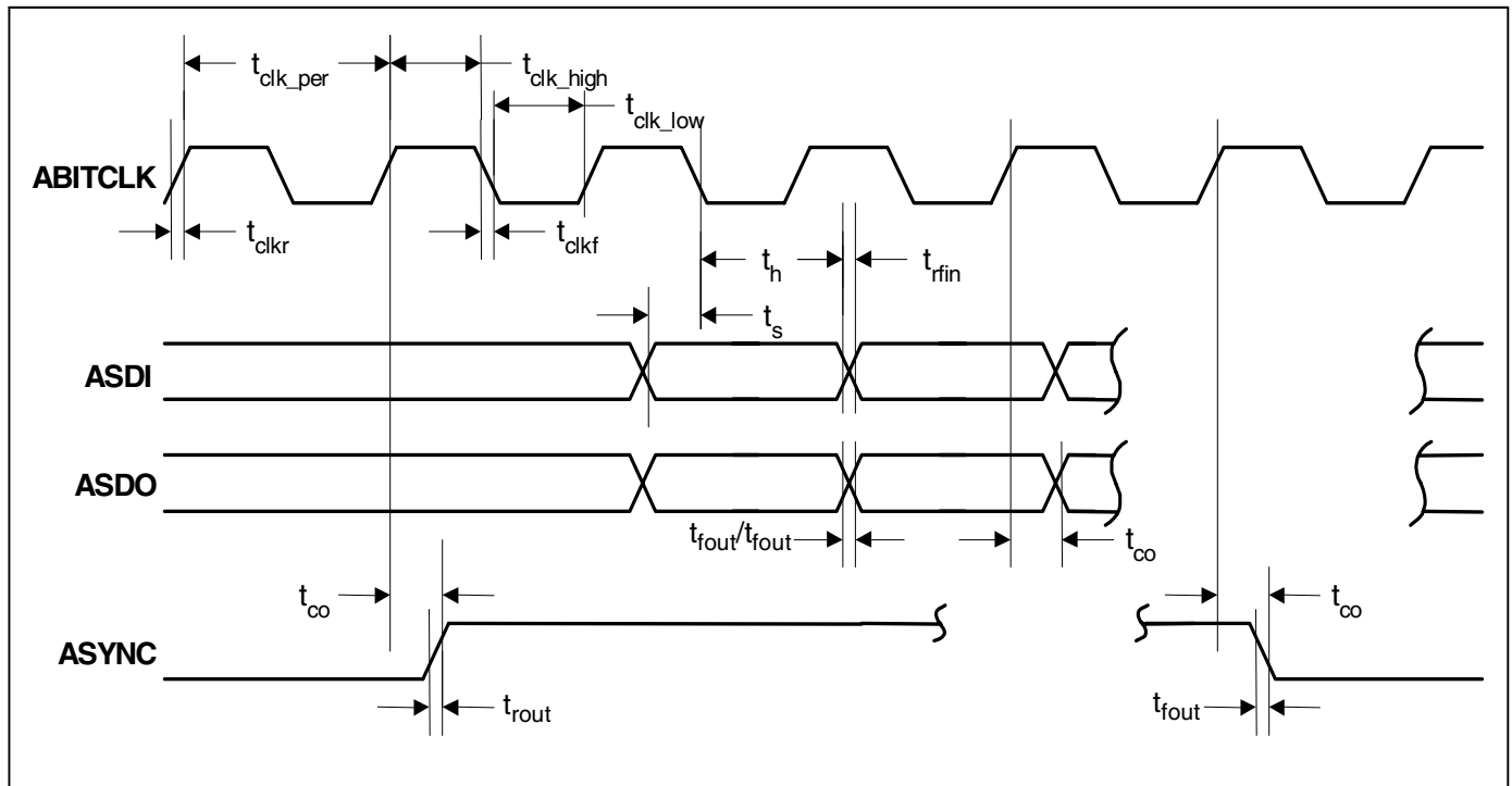
Figure 34. AC '97 Configuration Timing Measurement
