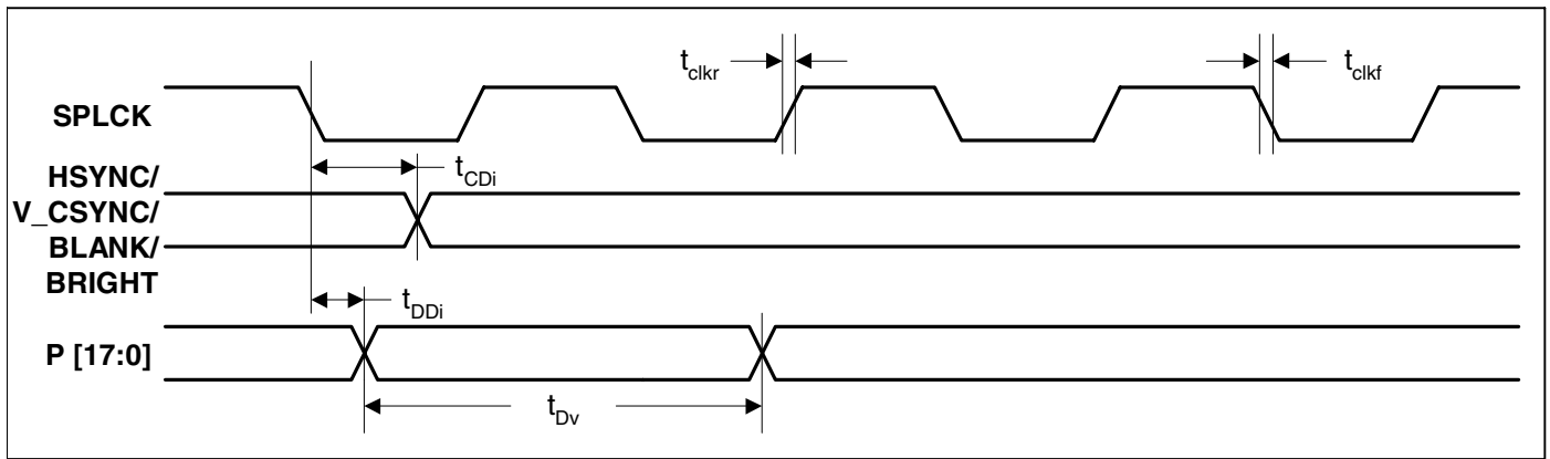
Figure 35. LCD Timing Measurement
