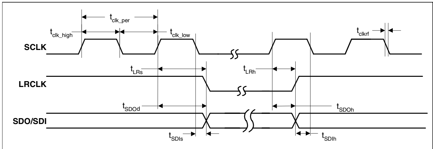
Figure 33. Inter-IC Sound (I 2 S) Timing Measurement
