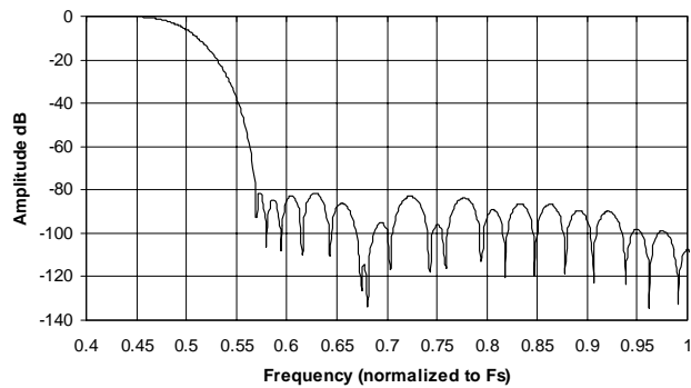
Figure 11. Double-speed Stopband
