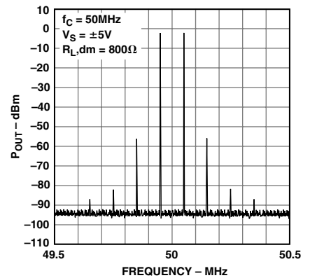
Figure 16. Intermodulation Distortion
