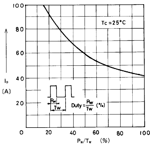
Current Duty Characteristics
