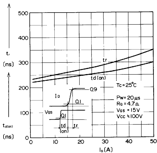
Turn-ON Characteristics
