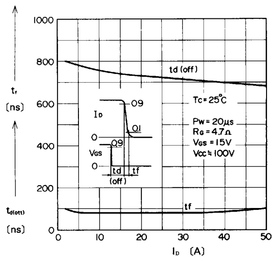
Turn-OFF Characteristics
