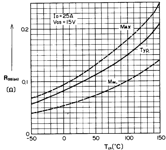
R_{DS(on)} - T_{ch} Characteristics
