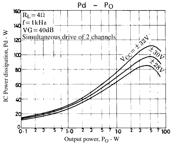
Figure 2. STK4181V Pd - P O (R L = 4Ω)
