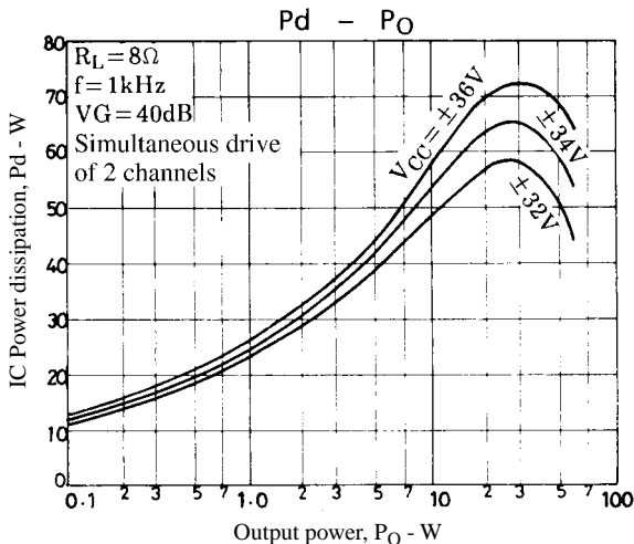
Figure 1. STK4181V Pd - P O (R L = 8Ω)
