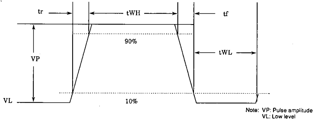
Fig. 3 Pulse Waveform
