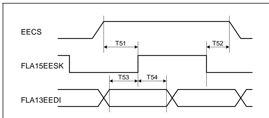
Figure 26. EEPROM Timings
