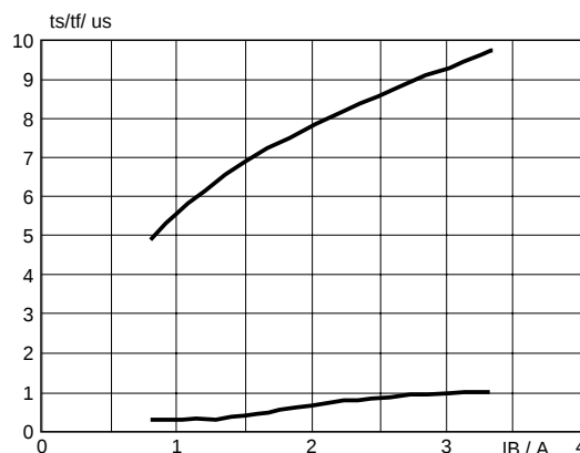
Fig.10. Limit storage and fall time. t_s = f(I_B) ; t_f = f(I_B) ; T_{HS} = 85^\circ\text{C} ; f = 16\text{ kHz}
