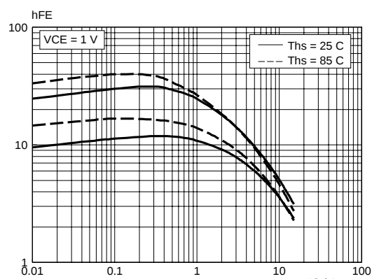
Fig.7. DC current gain. h_{FE} = f(I_C) Parameter T_{HS} (Low and high gain)
