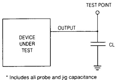
Figure 4. Test Circuit
