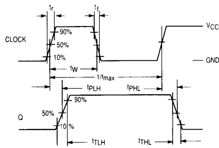
Figure 1. Switching Waveforms
