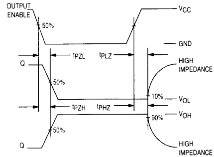
Figure 2. Switching Waveforms
