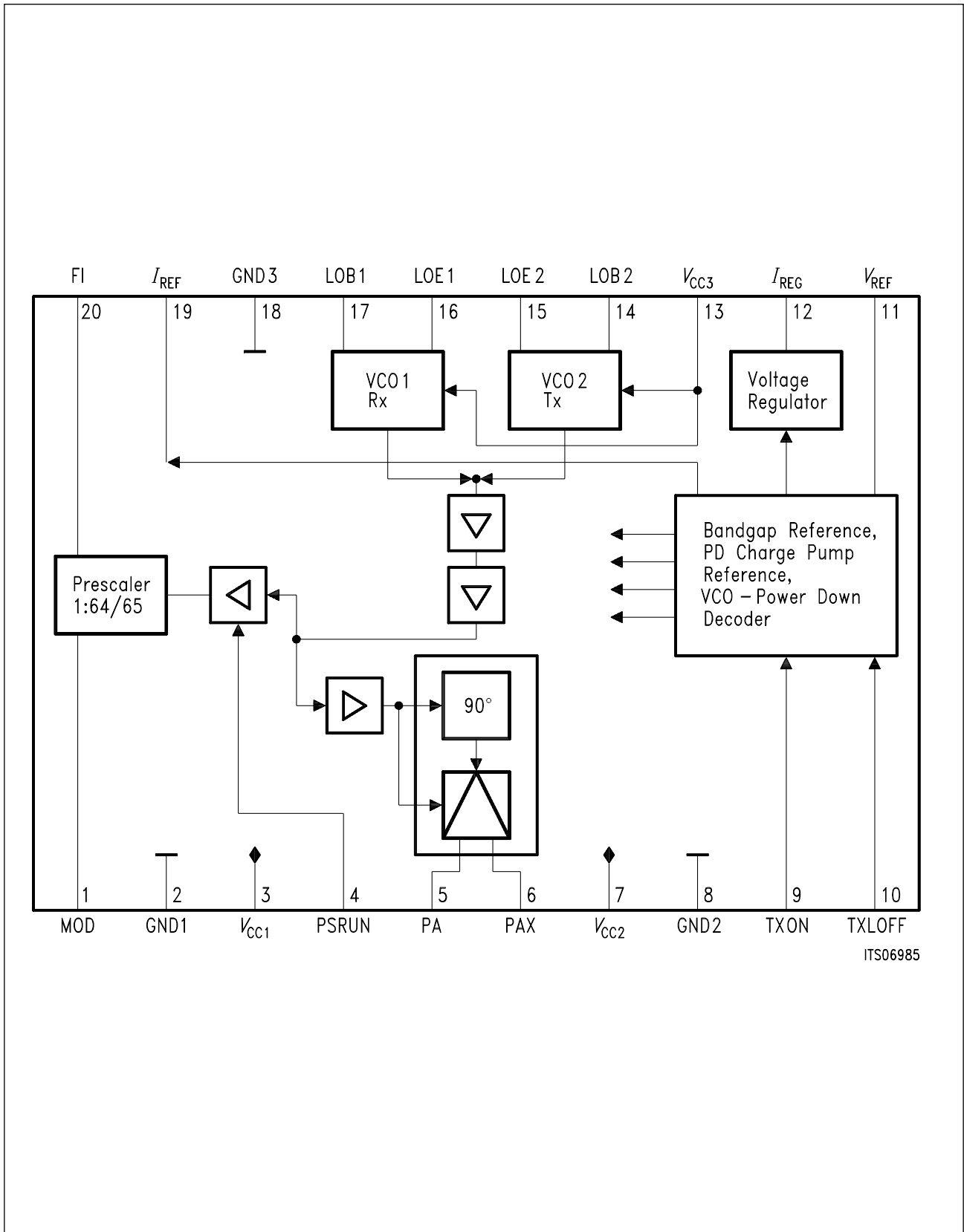
Figure 1 Block Diagram
