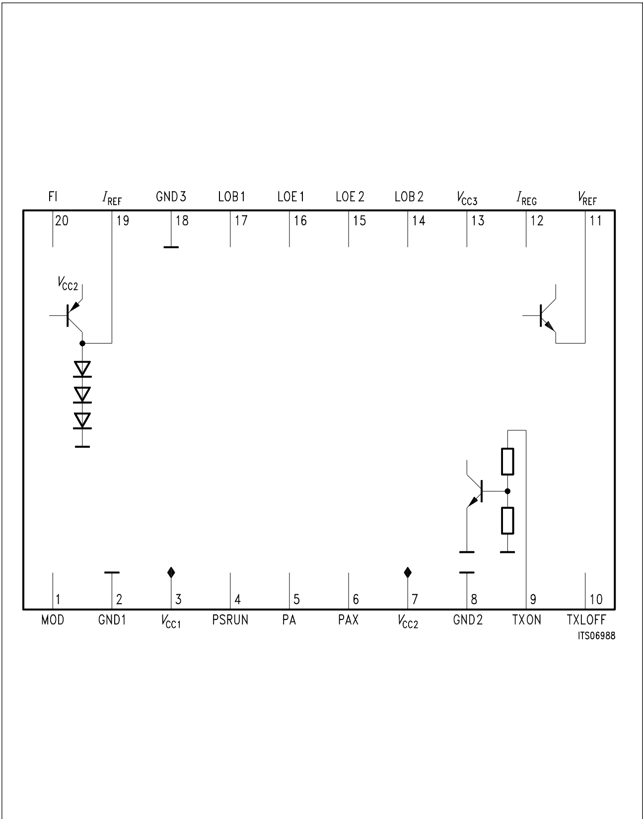
Figure 4 Input/Output Circuits Part 2
