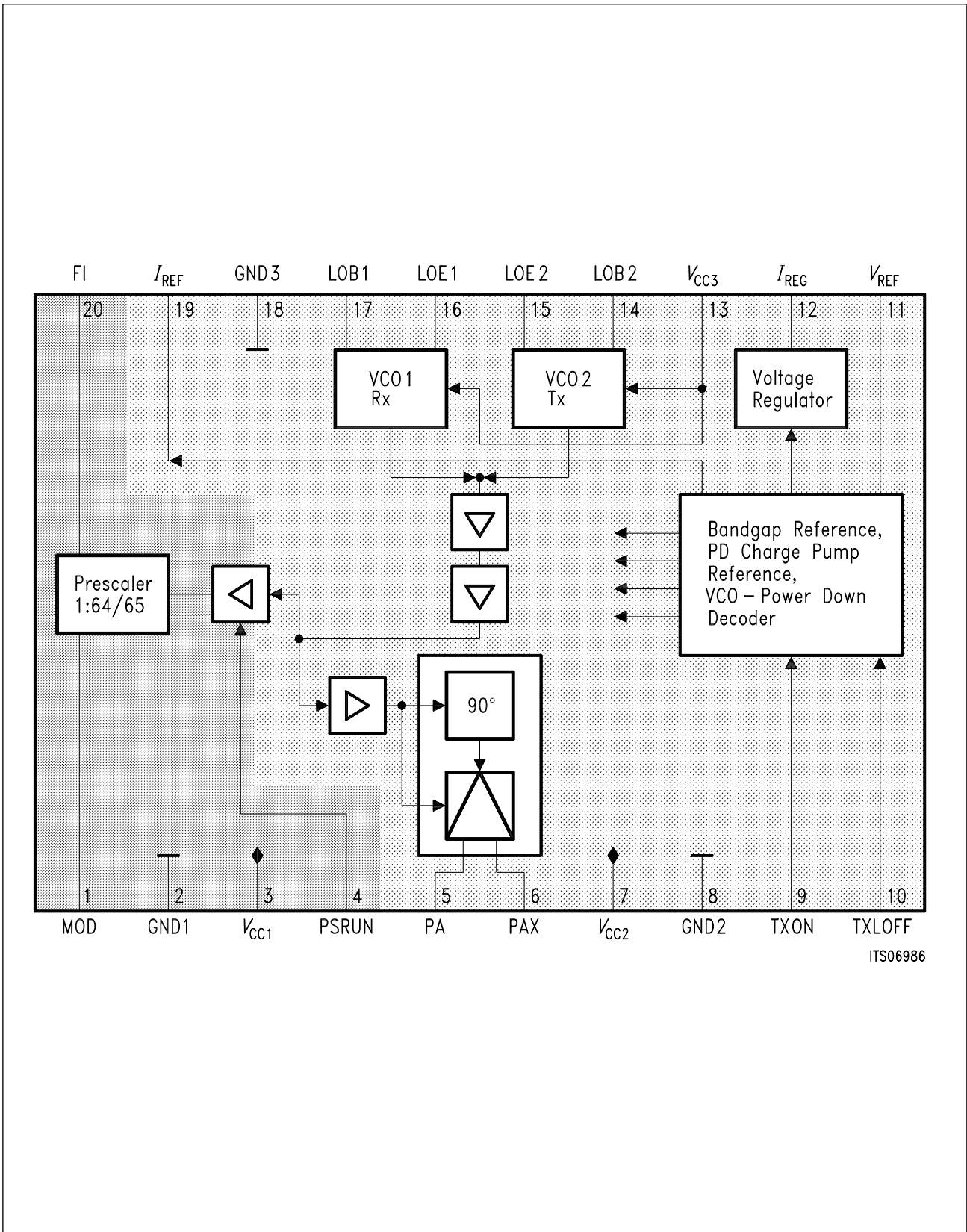
Figure 2 Supply Voltage Partitioning
