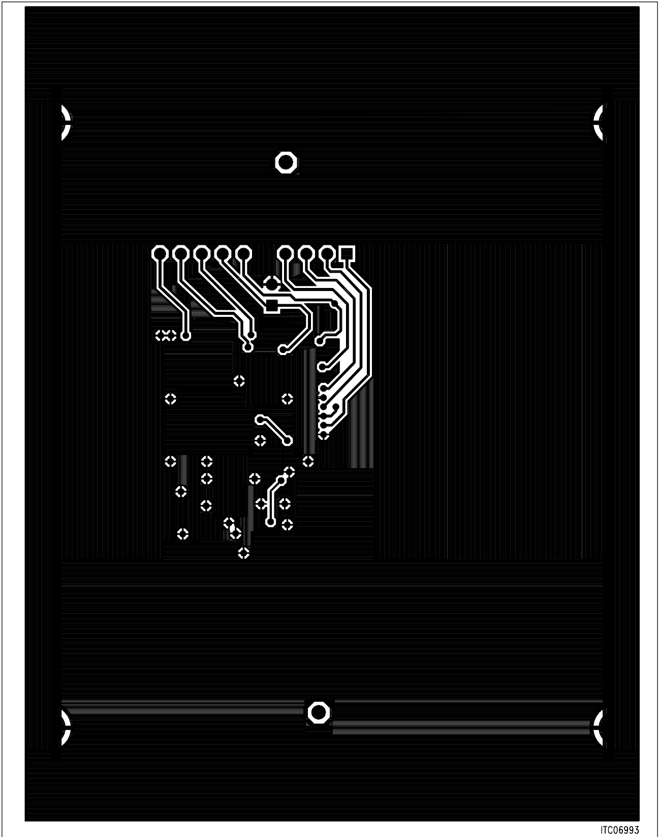
Figure 9 Test Circuit 2: Bottom Layer
