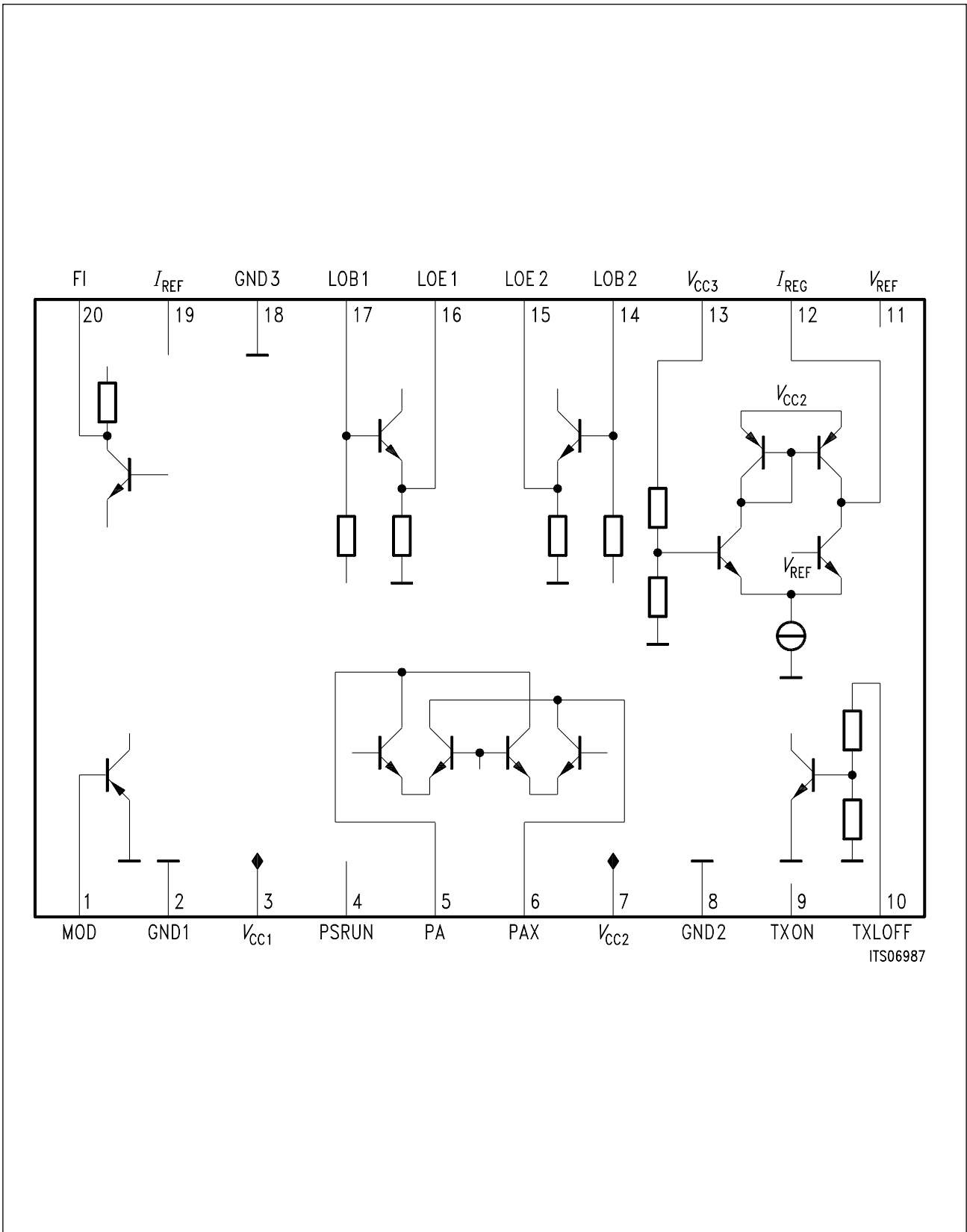
Figure 3 Input/Output Circuits Part 1
