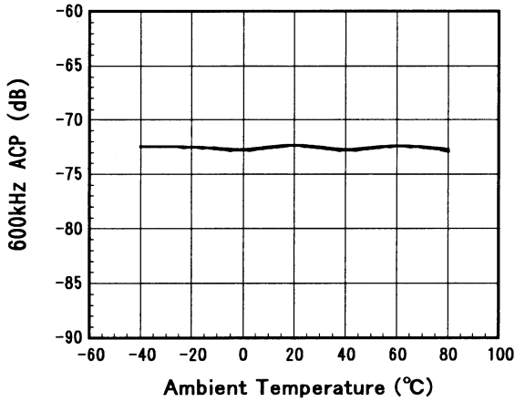
600kHz ACP vs. Temperature ( V_{CT1}=0V/2.7V , f_{i1}=1.9GHz , P_{i1}=0dBm )
