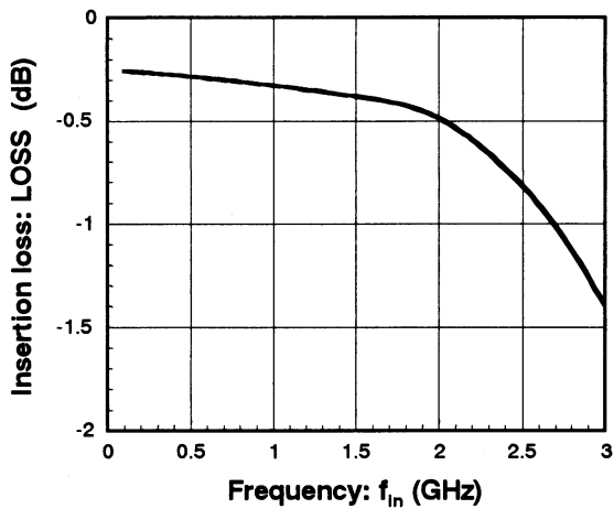
(PC-P1) Insertion loss vs. Frequency ( V_{CTR}=0V/2.7V , P_{in}=0dBm )
