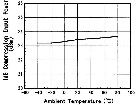
P-1dB vs. Temperature ( V_{CT1}=0V/2.7V , f_{i1}=2GHz )
