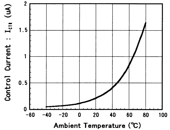
Control Current vs. Temperature ( V_{CT1}=0V/2.7V , f_{i1}=2GHz , P_{i1}=10dBm )
