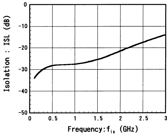
(PC-P1) Isolation vs. Frequency ( V_{CTR}=0V/2.7V , P_{in}=0dBm )
