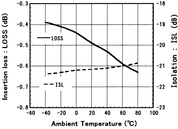
Loss/Isolation vs. Temperature ( V_{CT1}=0V/2.7V , f_{i1}=2GHz )
