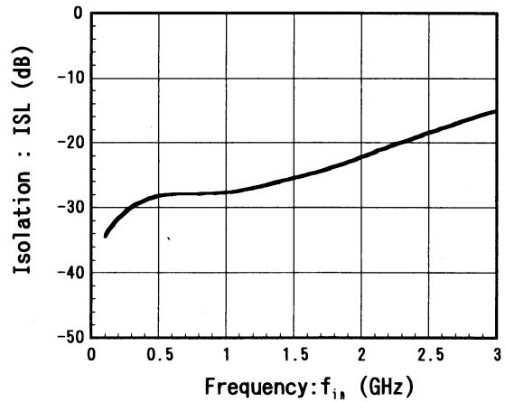
(PC-P2) Isolation vs. Frequency ( V_{CTR}=0V/2.7V , P_{in}=0dBm )
