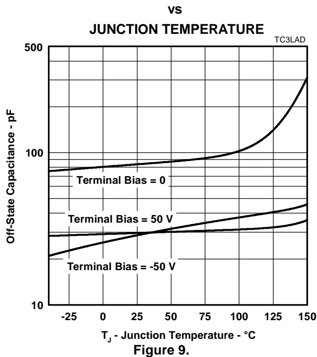
OFF-STATE CAPACITANCE
