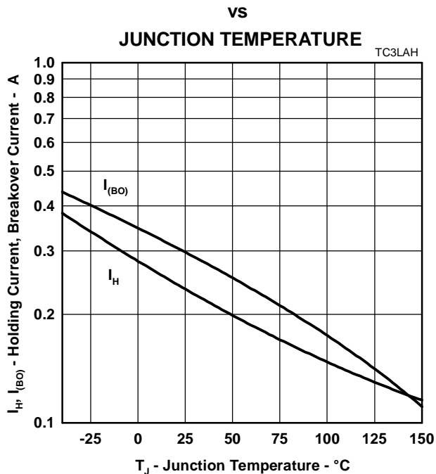
HOLDING CURRENT & BREAKOVER CURRENT
