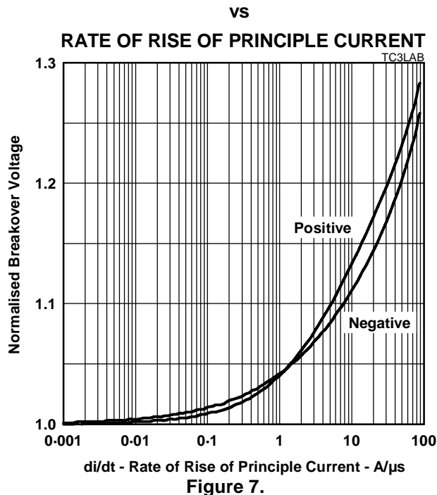
NORMALISED BREAKOVER VOLTAGE
