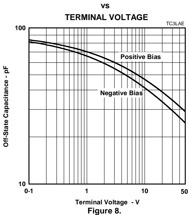
OFF-STATE CAPACITANCE
