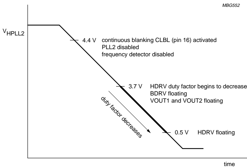
b. PLL2 shut-down sequence.
