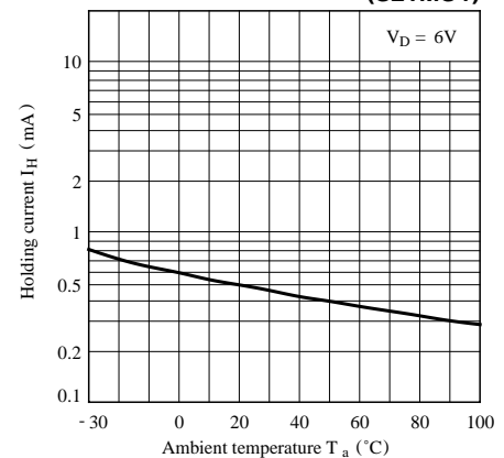
Fig. 7-b Holding Current vs. Ambient Temperature (S21MS4)
