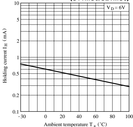
Fig. 7-a Holding Current vs. Ambient Temperature (S11MS3/S21MS3)
