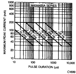
Fig. 8. Max Peak Current vs. Duty Cycle
