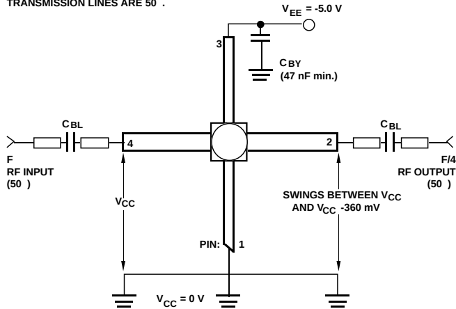
Figure 9. Typical ECL Biasing Configuration, IFD-53010 and IFD-53110.
