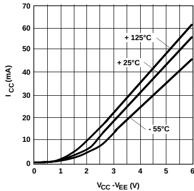
Figure 4. Device Current vs. Voltage and Temperature.
