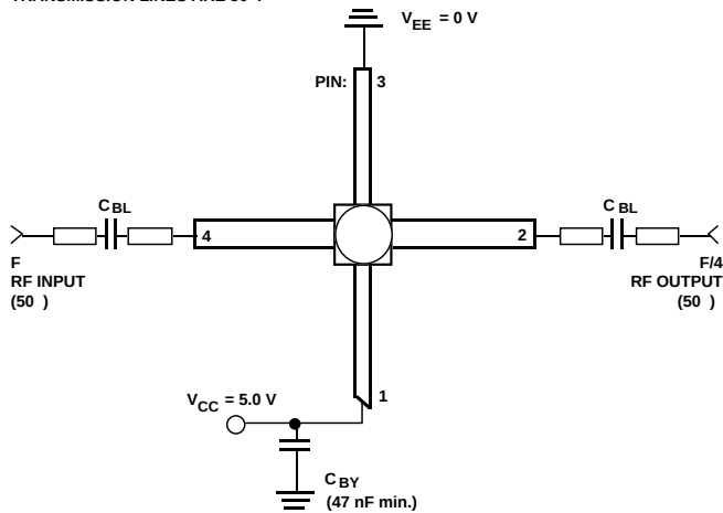
Figure 10. Typical RF Biasing Configuration, IFD-53010 and IFD-53110.
