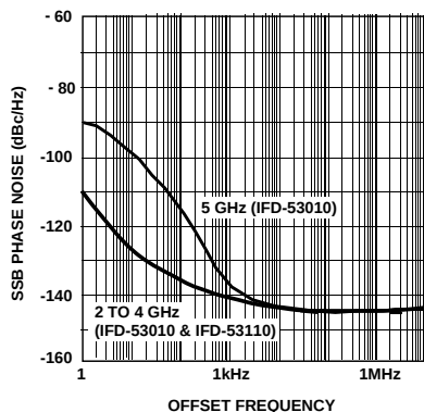
Figure 7. SSB Phase Noise vs. Offset Frequency, and Input Frequency.
