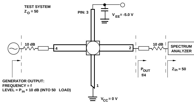
Figure 12. Sensitivity Test Configuration, IFD-53010 and IFD-53110.
