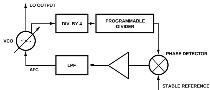
Figure 11. Typical Stabilized LO Configuration, IFD-53010 and IFD-53110.
