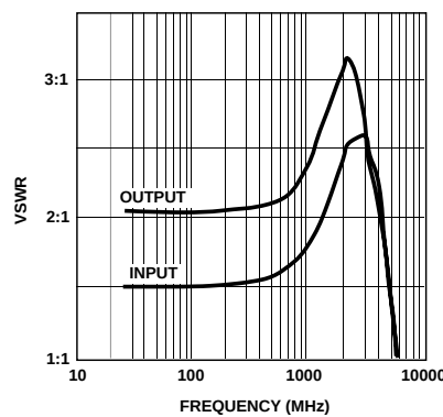
Figure 5. Input and Output VSWR vs. Frequency.
