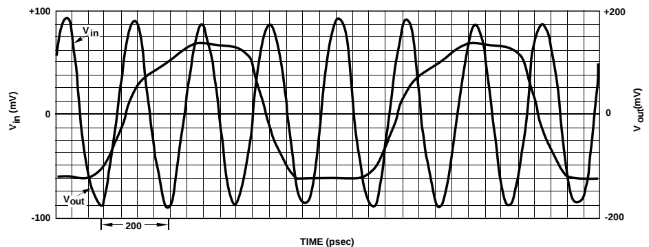
Figure 8. IFD-53010 Typical Output Response with 5 GHz Input.
