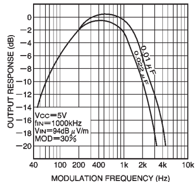
Fig. 4 AM fidelity characteristics
