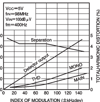
Fig. 25 Modulation characteristics
