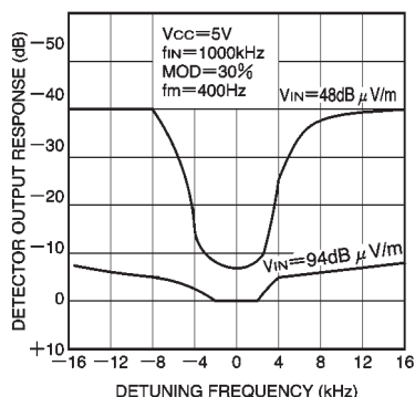
Fig. 18 Detuning characteristics
