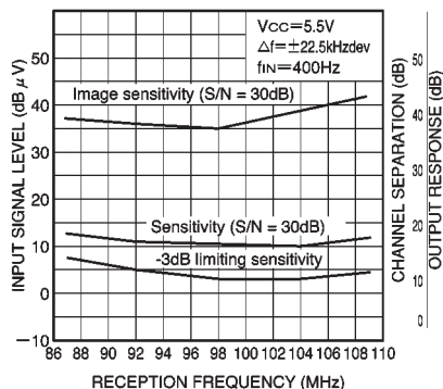
Fig. 23 Tracking characteristics
