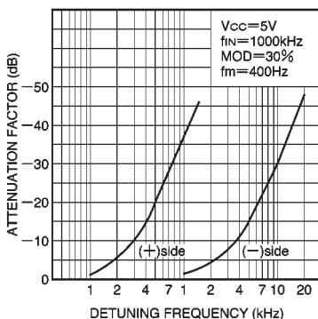
Fig. 17 Selectivity characteristics
