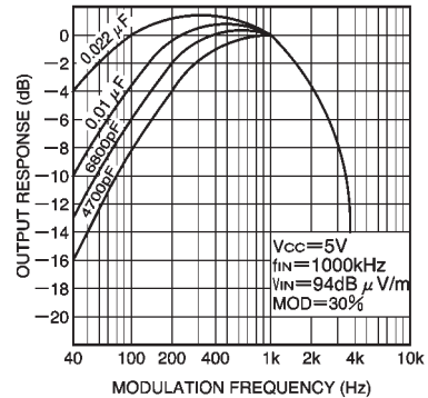
Fig. 3 AM fidelity characteristics
