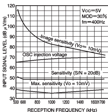
Fig. 14 Tracking characteristics
