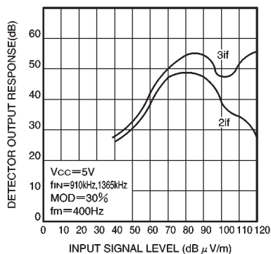
Fig. 20 Beat characteristics
