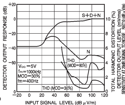
Fig. 21 Sensitivity characteristics
