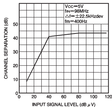
Fig. 28 Sensitivity characteristics
