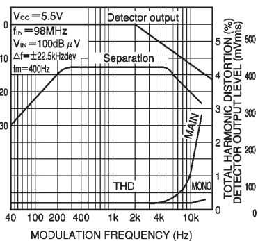
Fig. 24 Fidelity characteristics
