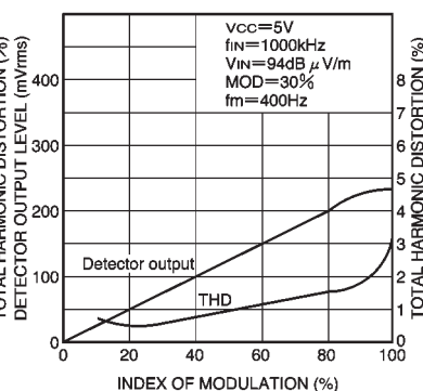
Fig. 16 Modulation characteristics
