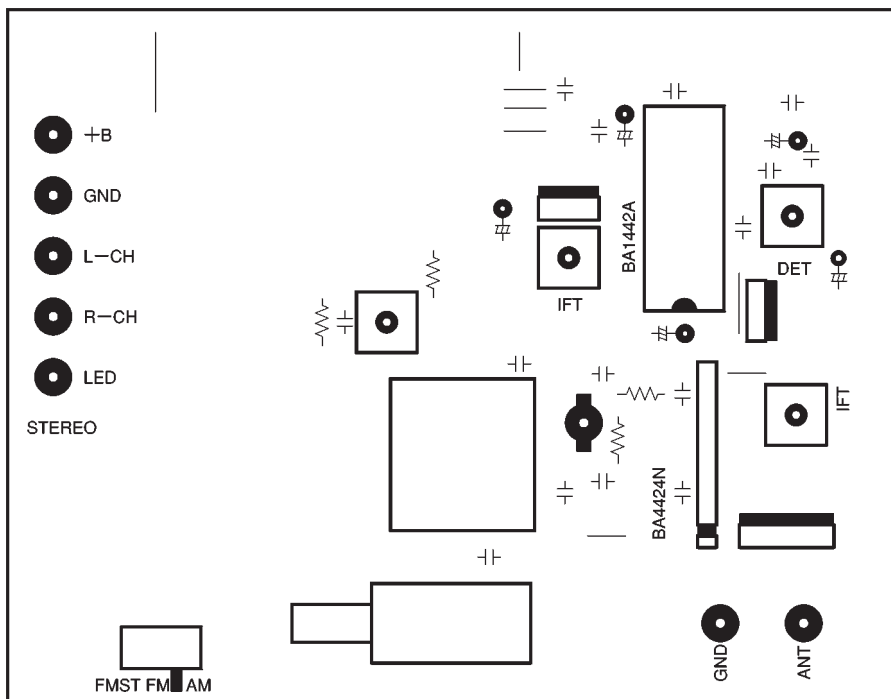
Component side
