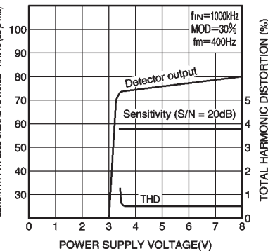
Fig. 22 Power supply voltage characteristics
