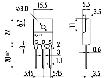
TO-3PF
