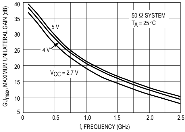
Figure 2. GU_{max} versus Frequency
