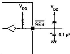
Figure 8. Reset input
