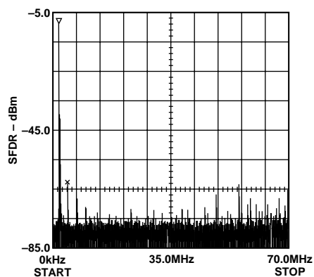
Figure 8. Single-Tone SFDR @ f_{CLOCK} = 140\text{ MHz} ( f_{OUT1} = 2\text{ MHz} )
