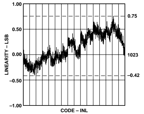
Figure 16. Typical Linearity
