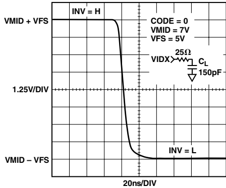
TPC 2. Invert Switching 10 V Step Response (Fall) at C_L
