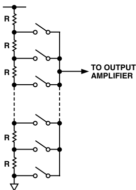
Figure 28. Resistor String
