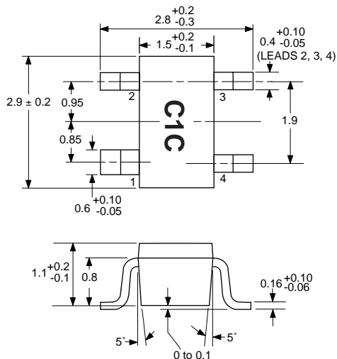
UPC1688G PACKAGE OUTLINE 39 (SOT-143)
