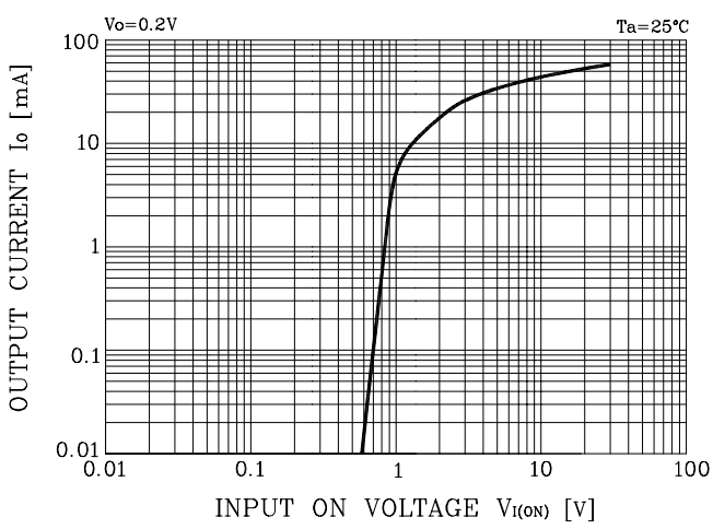
Fig. 1 I_o - V_{I(ON)}
