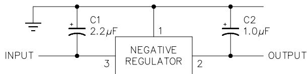
FIGURE 9 - FIXED OUTPUT REGULATOR
