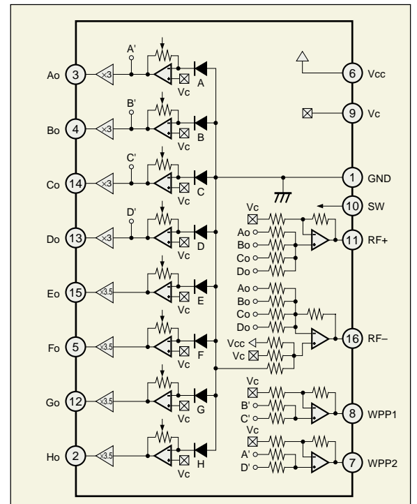
■ Figure 2 CXA2677GA Block Diagram
