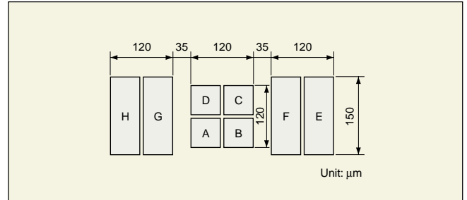
■ Figure 6 CXA2677GA Acceptance Pattern Dimensions
