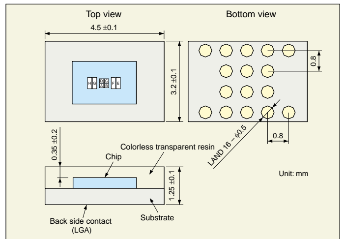
■ Figure 8 CXA2677GA Package Dimensions
