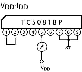
TEST CIRCUIT 2
