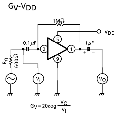
TEST CIRCUIT 3
