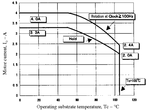
Figure 5. I_o - T_c
