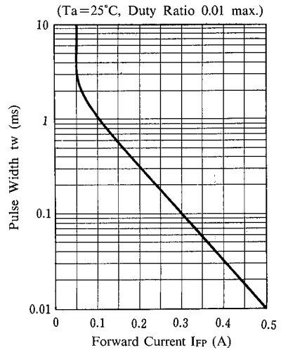
Pulse Width vs. Forward Current
