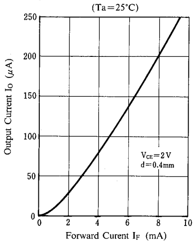
Output Current vs. Forward Current
