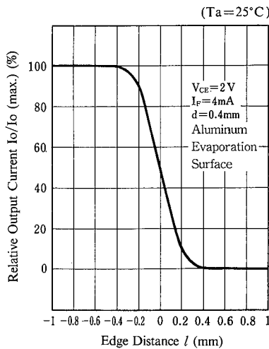
Output Current vs. Edge Distance (Ta=25°C)
