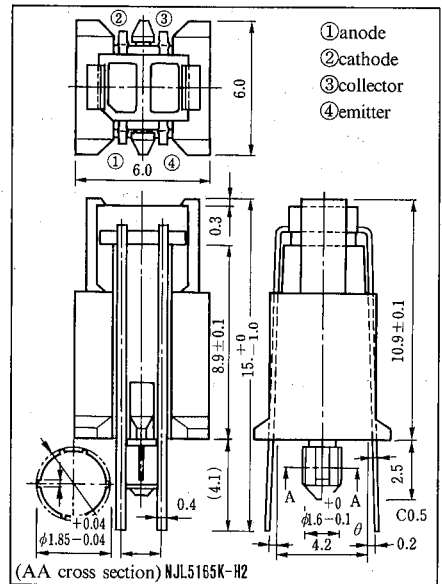
(AA cross section) NJL5165K-H2
