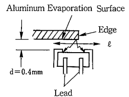
Measuring Specification for Edge Response
