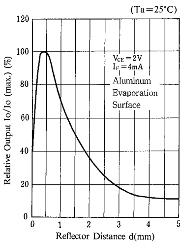
Output Current vs. Distance (Ta=25°C)
