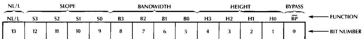
Figure 7. 14-Bit Latch
